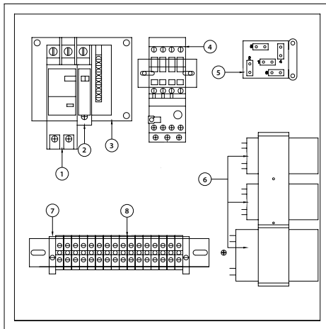
Airmax 230v Control Panel 5 HP
