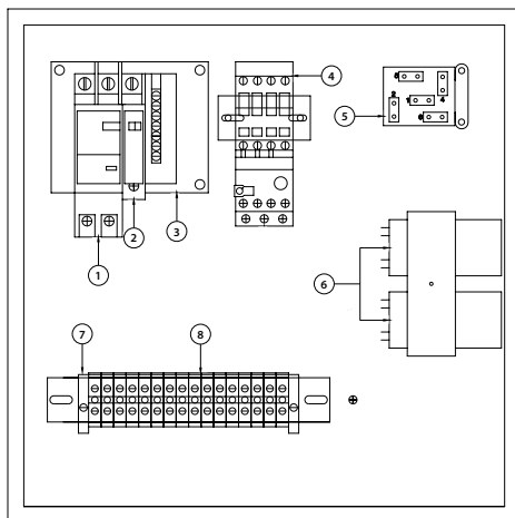
Airmax 230v Control Panel 1 HP
