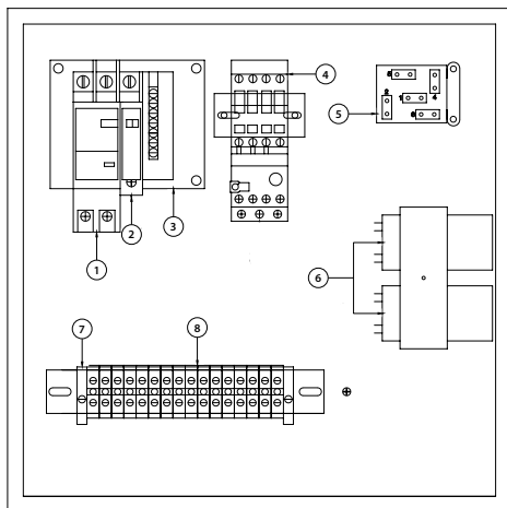
Airmax 230v Control Panel 3 HP
