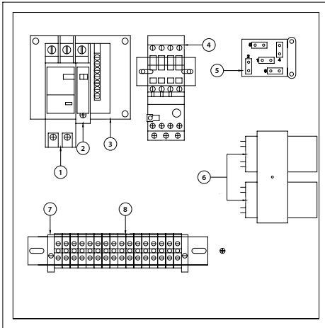
Airmax 230v Control Panel 2 HP
